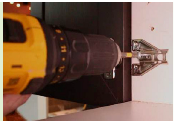
Front screw adjusts right and left. Back screw adjusts in and out.
